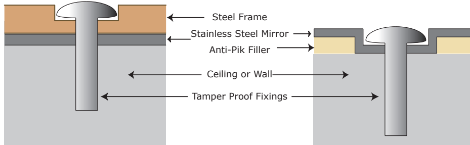
Counter-Sunk Hole in Frame
