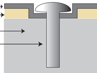
Counter-Sunk Hole in Stainless Steel Frameless Dome
